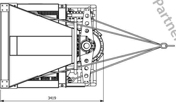
FRONT VIEW ( 1:50 )
