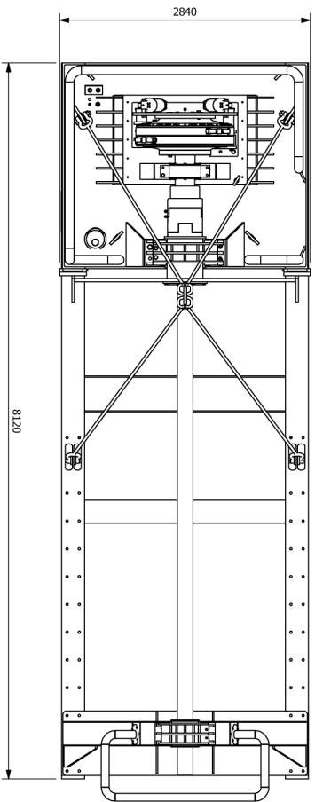
PLAN VIEW ( 1:50 )
